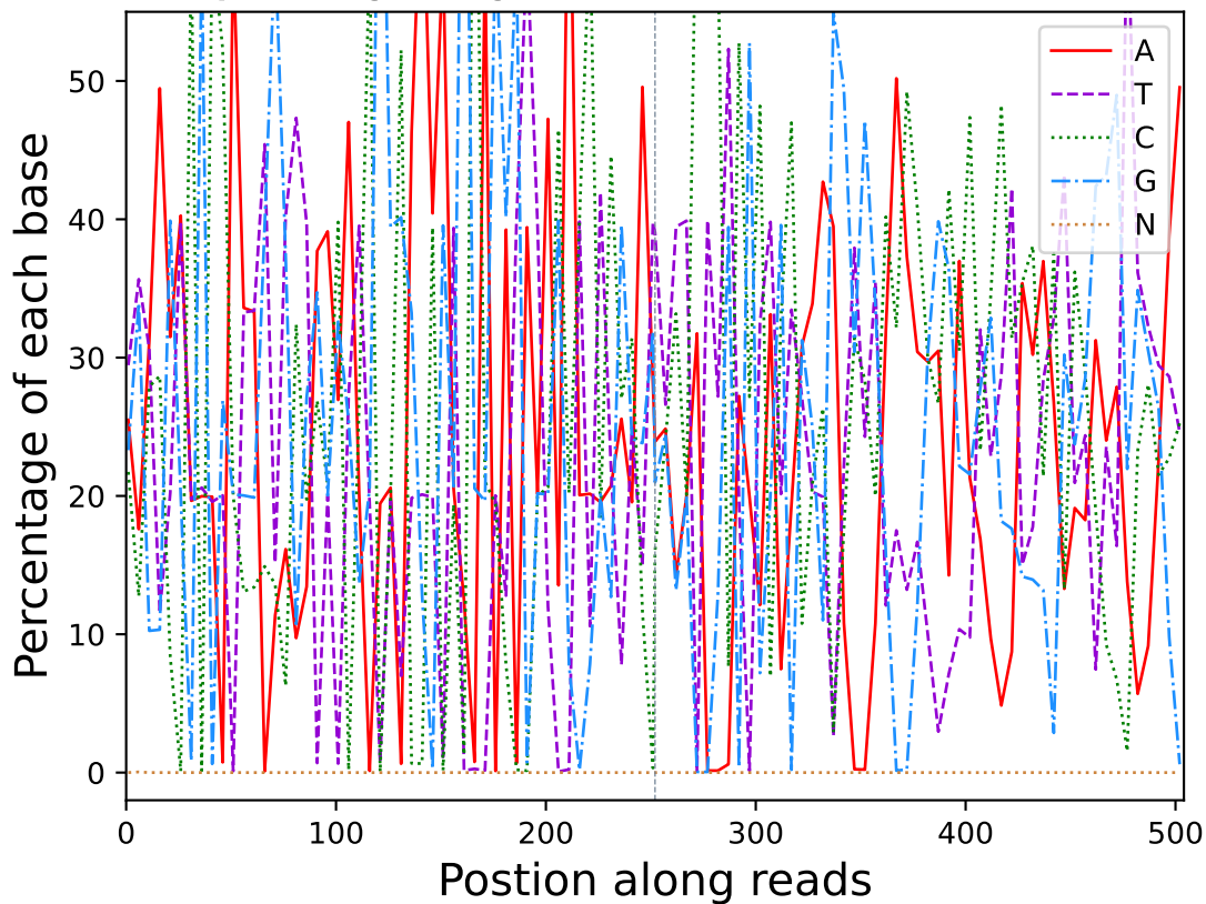
Base percentage along reads (R10305)
